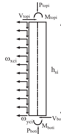
Fig. 7. In-plane free body diagram of the VBE at the i^{th} story for determination of shear demand.
