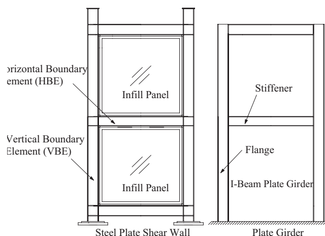
Fig. 1. Typical steel plate shear wall and analogous vertical cantilever plate girder.
