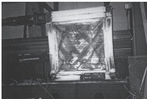
Fig. 6. Deformation and yield patterns of SPSW2 after 68\delta_y (Lubell et al., 2000).
