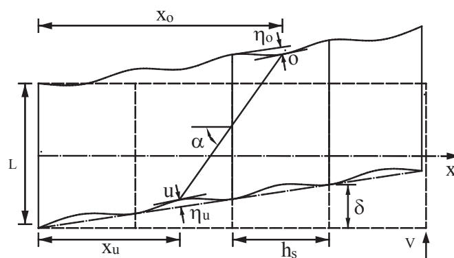
Fig. 2. Deformation of a cantilever plate girder under transverse load (adapted from Wagner, 1931).
