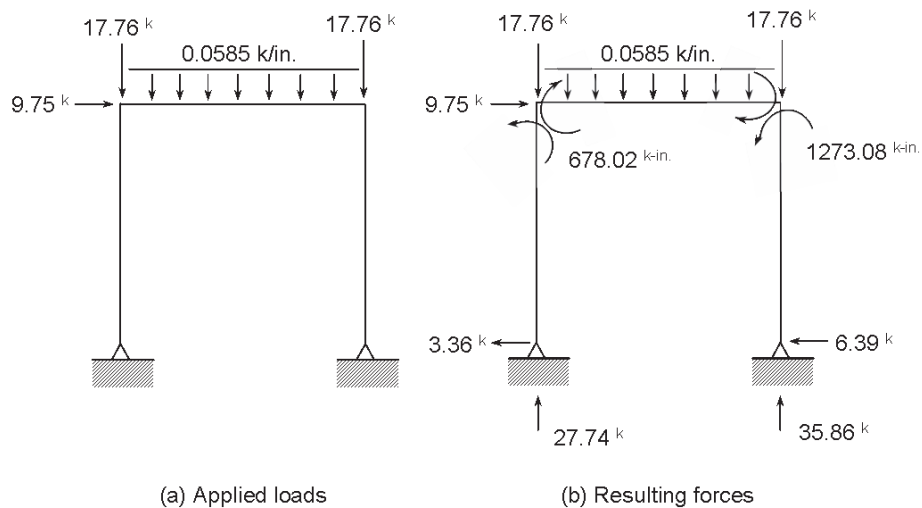
Fig. 6. Example of an EBT model for 1.2D + 1.3W + 0.5S .
