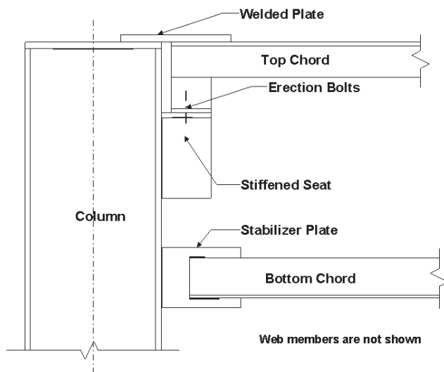
Fig. 9. Typical joist girder moment connection.
