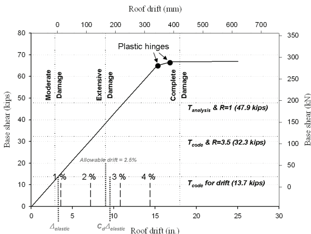
Fig. 13. Pushover curve for three-bay frame.
