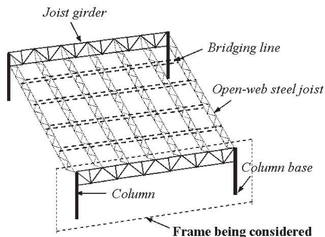
Fig. 1. One-bay, one-story steel joist girder structure.
