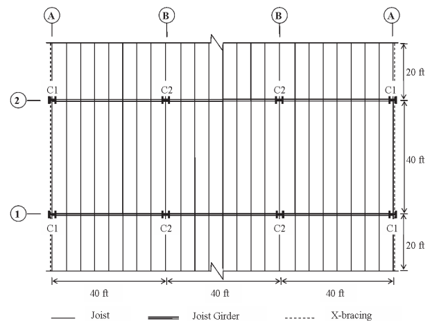
Fig. 3. Plan of a three-bay frame.
