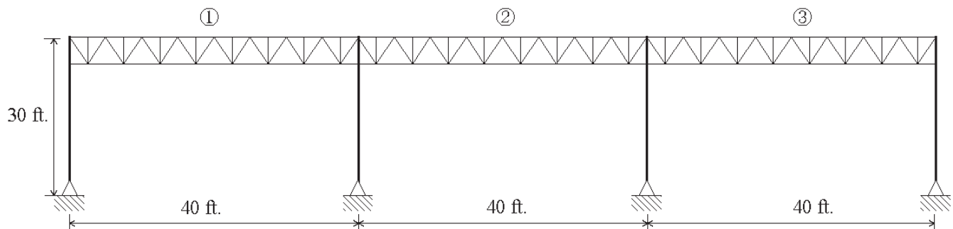
Fig. 4. Elevation of a three-bay frame.
