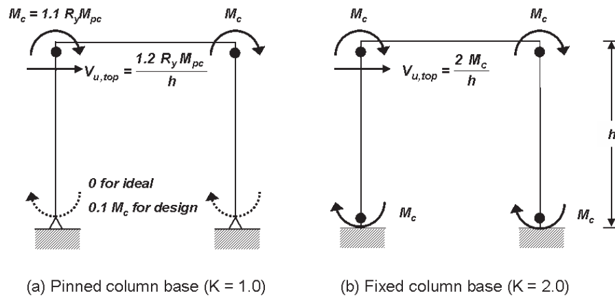
Fig. 8. Theoretical K factors for the column plastic capacity.
