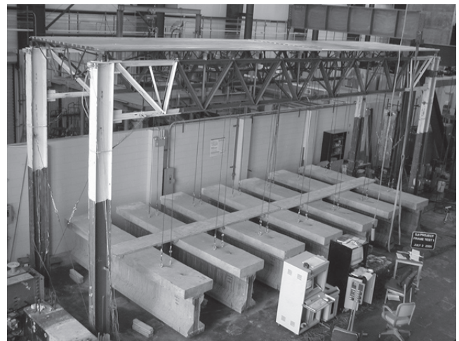
Fig. 10. Overview of test setup.
