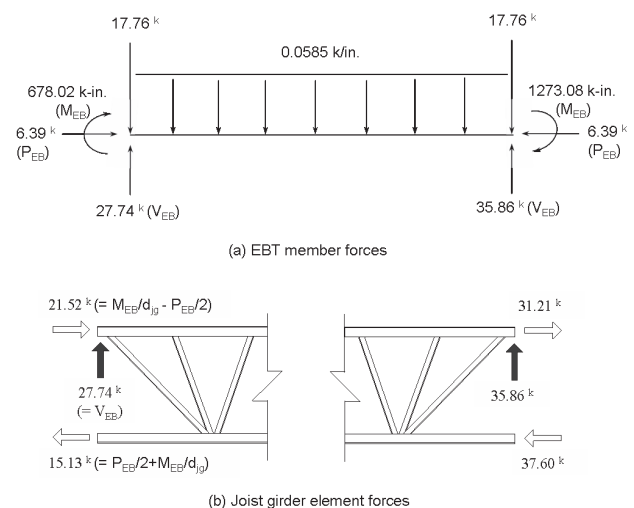
Fig. 7. Conversion of forces for 1.2D + 1.3W + 0.5S.
