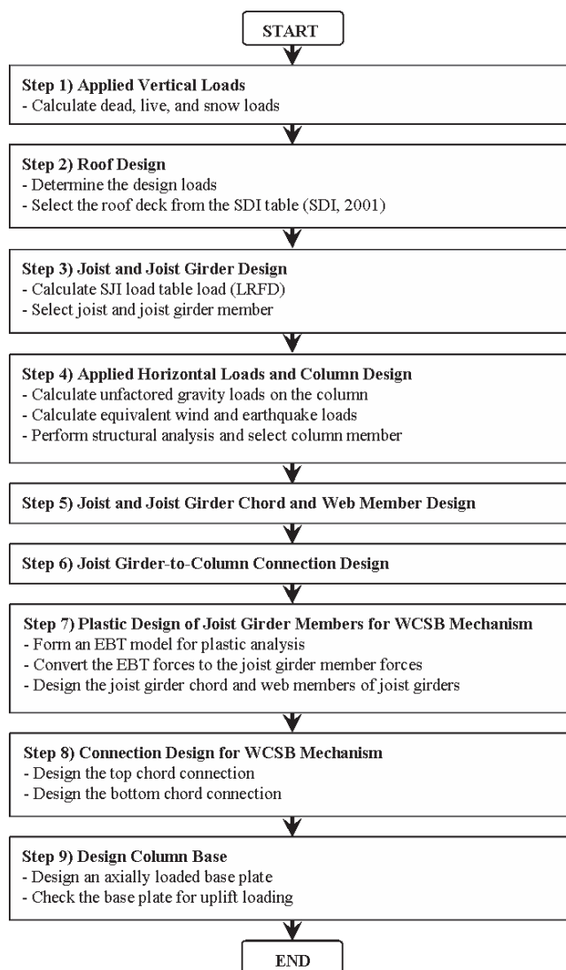
Fig. 2. Flowchart for proposed seismic design procedure.
