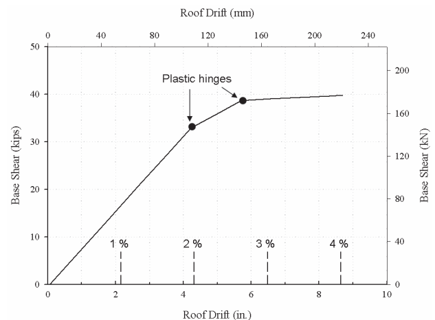
Fig. 12. Pushover curve for one-bay frame.
