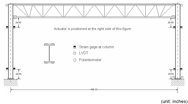
Fig. 6. Sensor locations.
