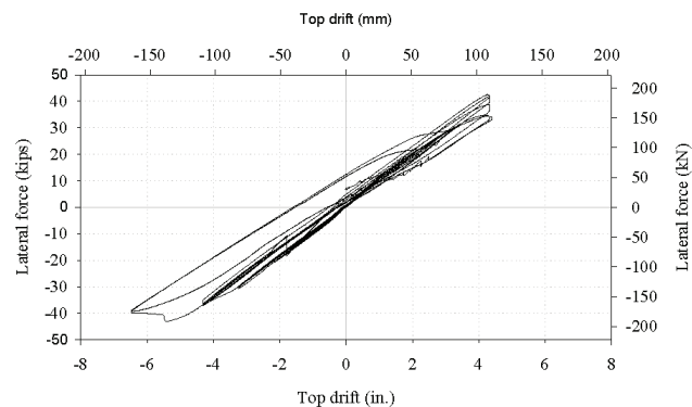
Fig. 8. Load-displacement curve of the test frame.
