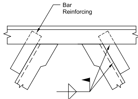
Fig. 10. Reinforcing diagonals.
