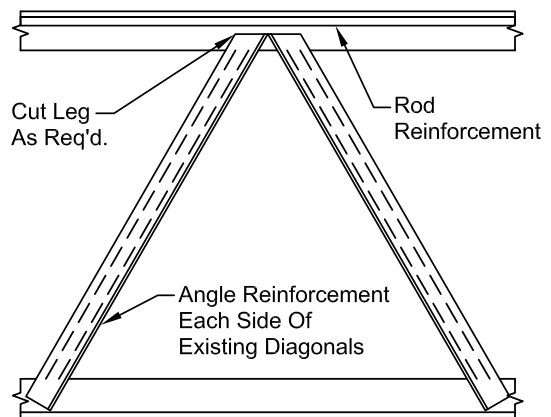
Fig. 6. Angle reinforcement on rod web joist.
