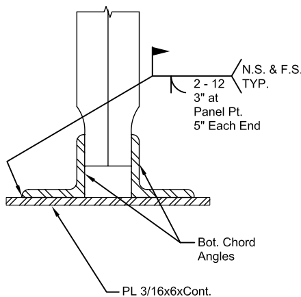
Fig. 22 Bottom chord reinforcement.
