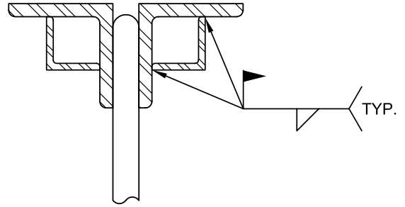
Fig. 2d. Top chord reinforcement—angles.
