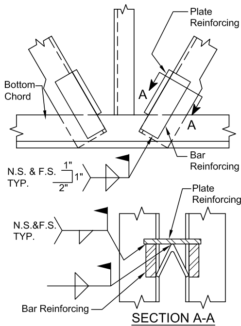
Fig. 11. Reinforcing diagonals.
