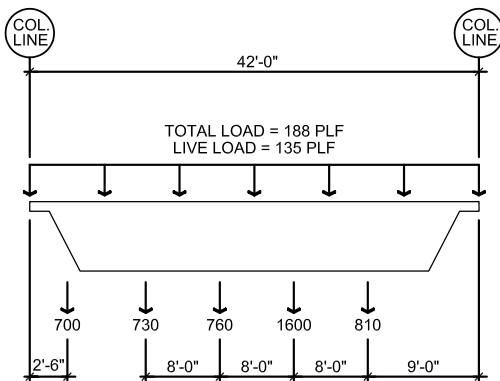
Fig. 19. Joist loading.
