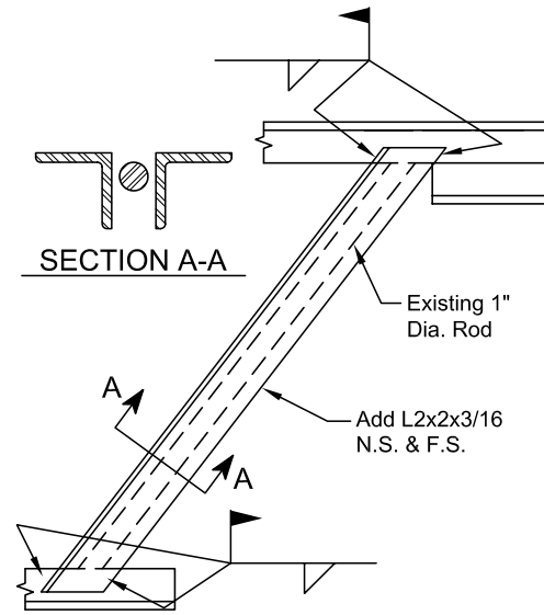
Fig. 17. Angles and welds added.
