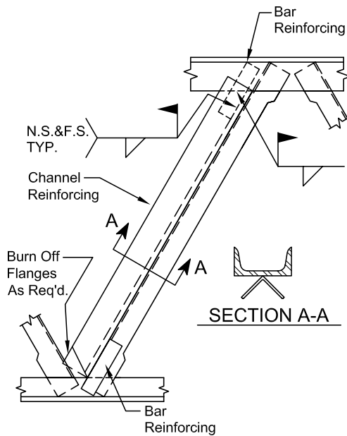
Fig. 12. Channel reinforcing.
