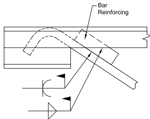
Fig. 18. Bar added for additional weld.
