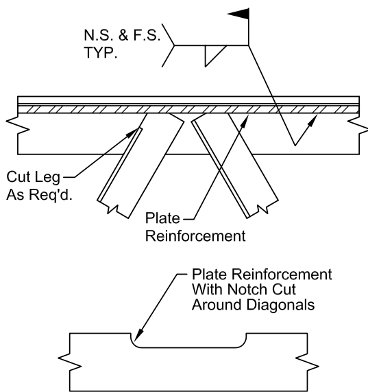
Fig. 4. Chord reinforcement requiring notch.
