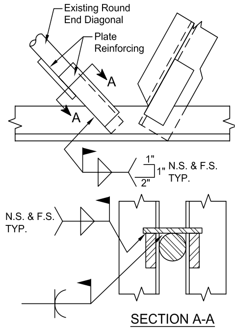
Fig. 13. Channel reinforcing at end diagonal
