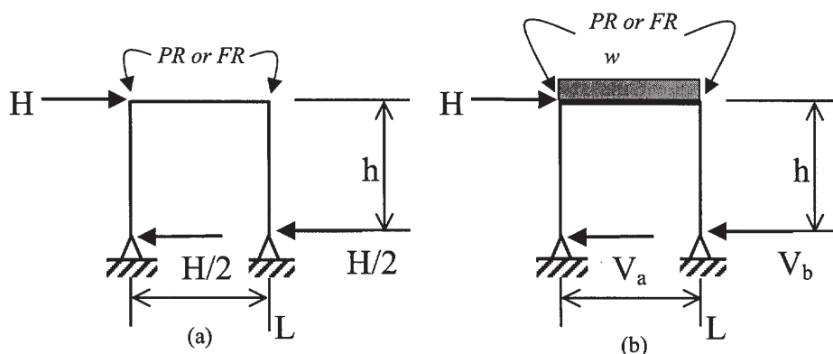
Fig. 5. Portal frame with lateral and gravity load.
