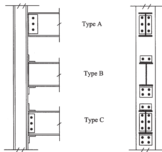
Fig. 12. Three types of semi-rigid connections.
