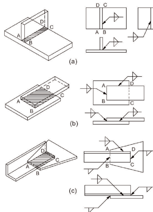
Fig. 6. Fillet Welds.
