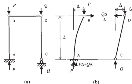
Fig. 9. Equilibrium Forces for Yura Derivation
