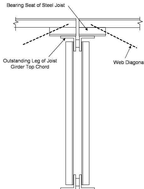
Fig. 1. Joist bearing on joist girder at panel point.
