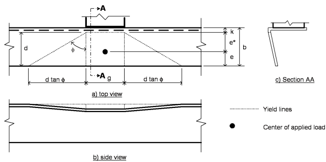
Fig. 6. Geometry of the plastic mechanism.
