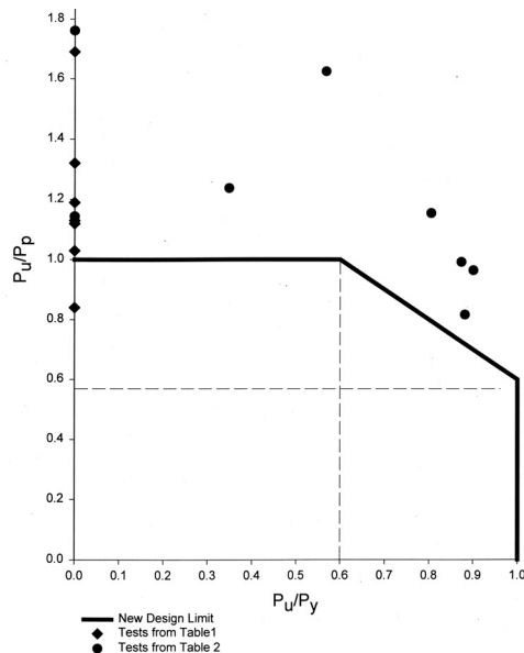
Fig. 11. Test results on the interaction space.
