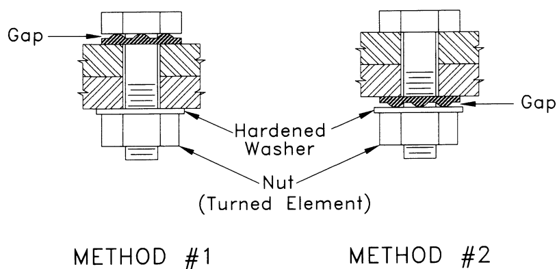
Fig. 1. (Revised) DTI Installation Methods
