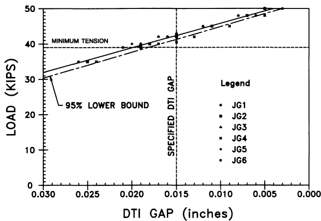
Fig. 18. F959-96 Annex A1—Load vs. DTI Gap, 7/8-in. A325 Galvanized Steel Bolts with Galvanized DTIs, MFR #1
