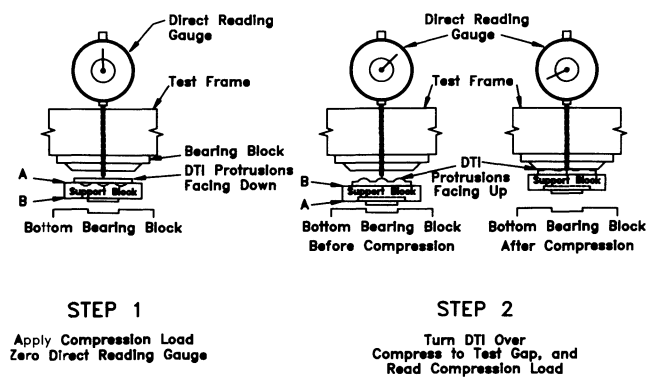
Fig. 15. ASTM F959-96 Annex A1 Test Assemblies
