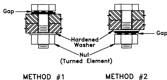
Fig. 1. DTI Installation Methods
