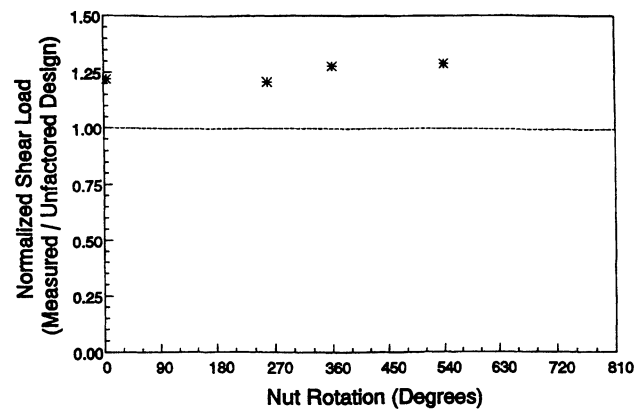
Fig. 12. Normalized Eccentric Single Shear vs. Nut Rotation, 7/8-in. A325 Weathering Steel, 3.5 in. Grip Length
