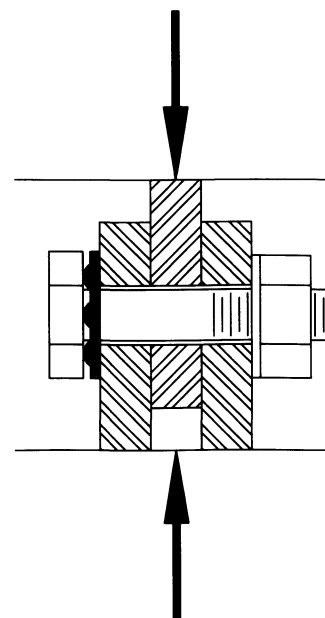
Fig. 2. Concentric Compressive Double Shear Apparatus
