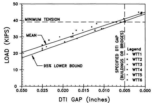
Fig. 7. Bolt Tension vs. Average DTI Gap, 7/8-in. A325 Weathering Steel Bolts with Epoxy Coated DTIs
