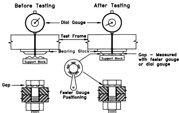
Fig. 14. ASTM F959-90 Test Assemblies
