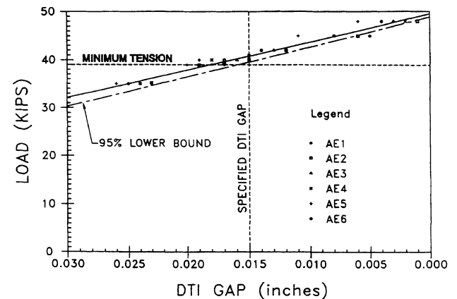
Fig. 21. F959-96 Annex A1—Load vs. DTI Gap, 7/8-in. A325 Weathering Steel Bolts with Epoxy Coated DTIs, MFR #2
