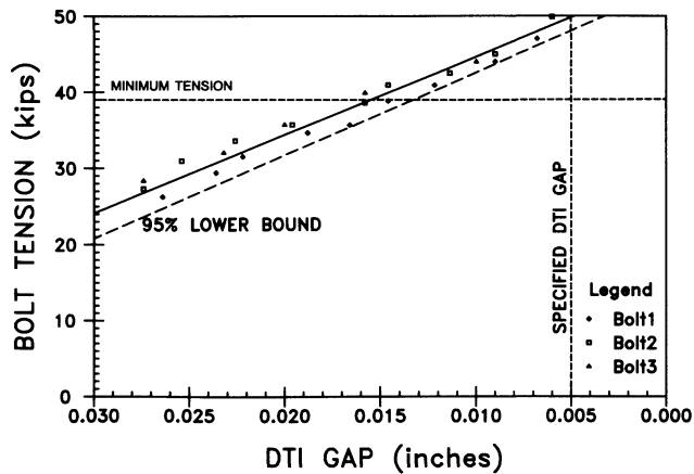
Fig. 24. Bolt Tension vs. Average DTI Gap, Field Tests 7/8-in. A325 Galvanized Bolts with Galvanized DTIs, MFR #1
