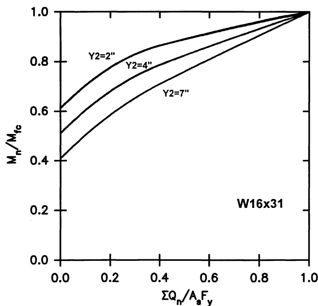
Fig. 2. Normalized moment versus percent shear connection.
