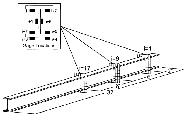
Fig. 6. Strain gage locations for composite beam specimens.
