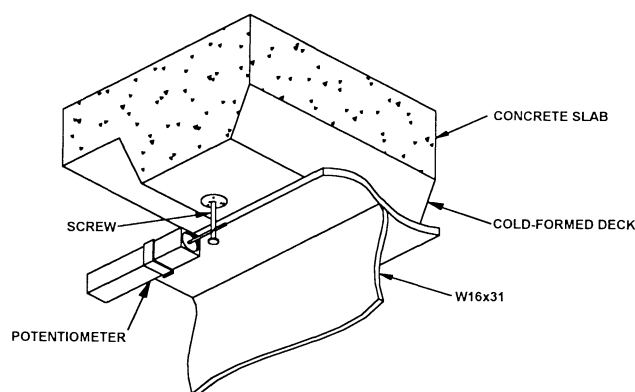
Fig. 7. Slip measurement detail.
