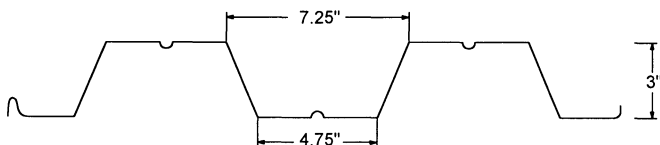
Fig. 3. Composite deck profile.
