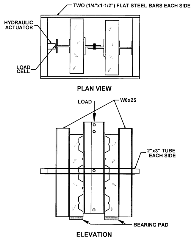
Fig. 10. Push-out specimen schematic.
