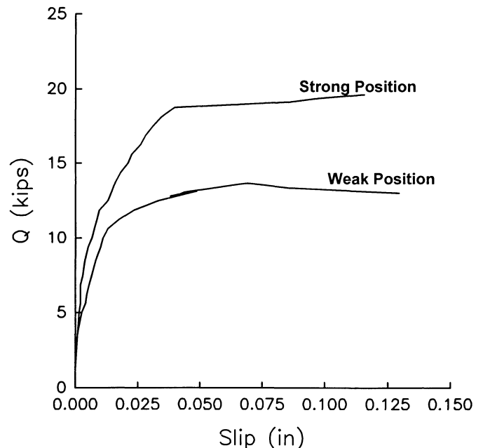
Fig. 12. Load vs. slip for strong and weak position shear studs for push-out tests.
