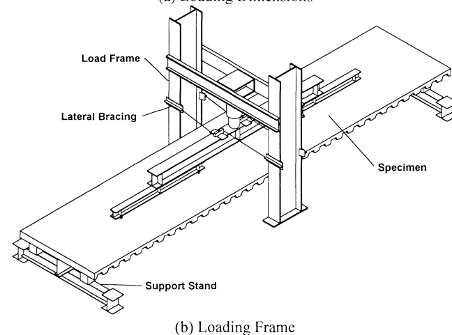
Fig. 9. Loading frame for composite beam specimens.
