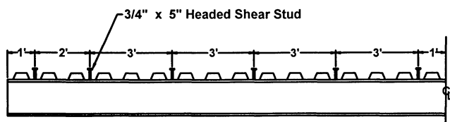
Fig. 4. Shear stud locations for composite beam specimens.
