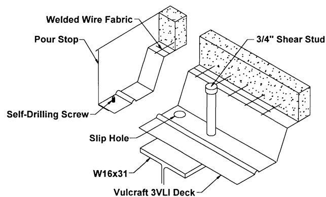
Fig. 5. Deck/slab detail.
