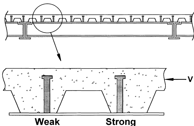
Fig. 1. Strong and weak position shear stud locations.
