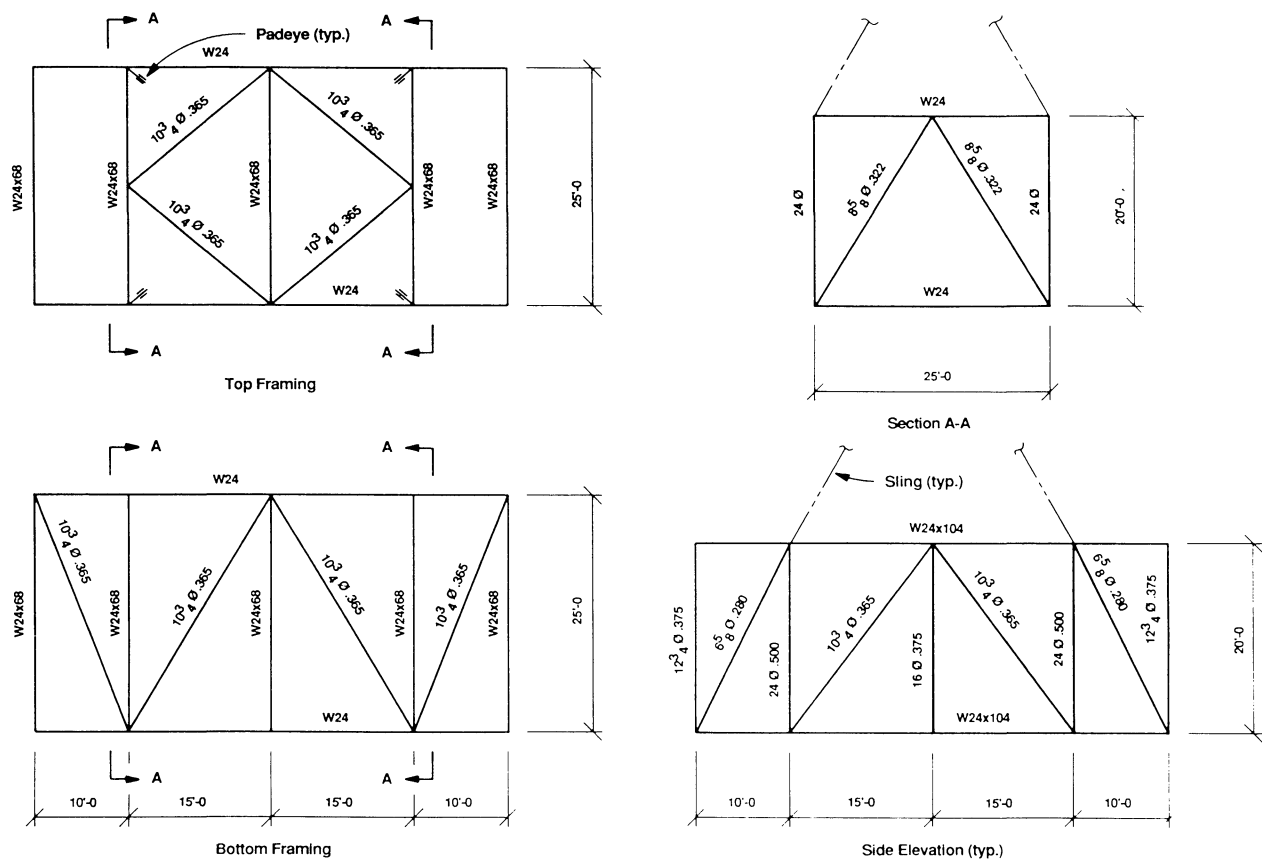
Fig. 1. Module framing plans and elevations.
