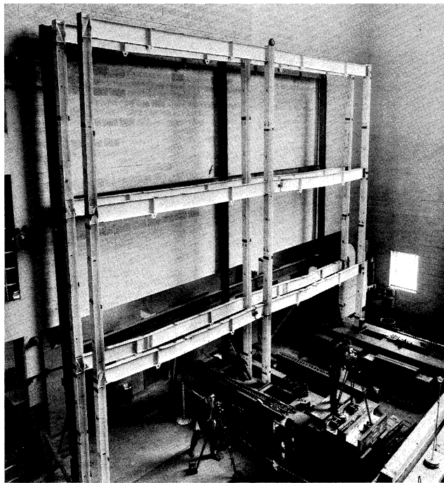
Fig. 16. Braced frames after testing
