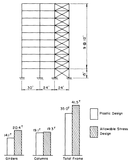
Fig. 1. Weight comparison for plastic design and allowable stress design
