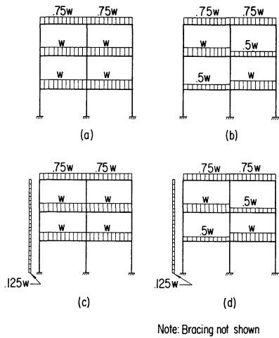
Fig. 2. Loading conditions for braced frame tests
