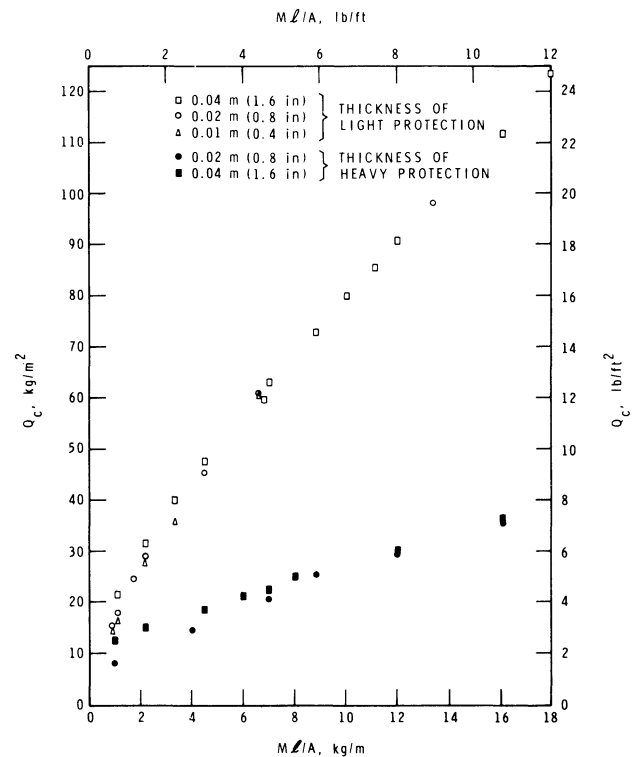
Fig. 8. Critical fire load as a function of M/A for a large opening factor ( F = 0.18 \text{ ft}^{1/2} )
