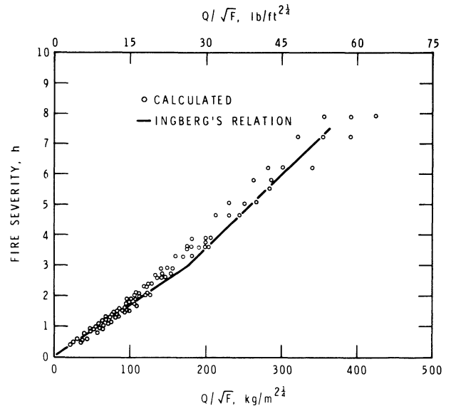
Fig. 12. Comparison of Ingberg's relation with calculated values
