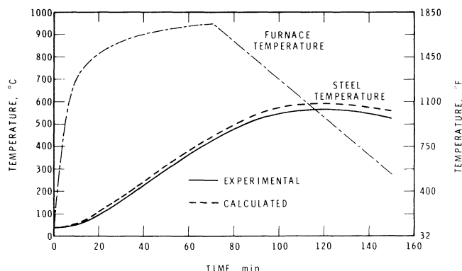
Fig. 5. Steel and furnace temperature as a function of time (size steel core: 10 in. X 10 in.; insulation of vermiculite board)
