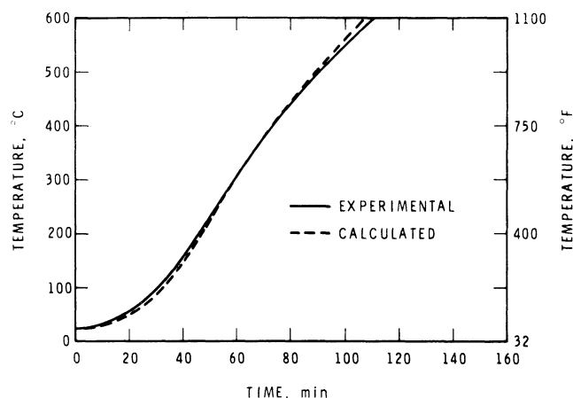
Fig. 4. Steel temperature as a function of time (size steel core: 8 in. X 8 in.; insulation of heavy clay brick)
