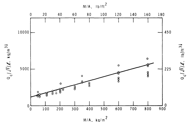
Fig. 10. Relation of factors that determine the fire resistance of protected steel (heavy protection)
