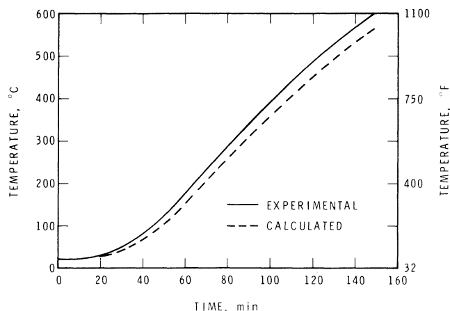
Fig. 3. Steel temperature as a function of time (size steel core: 6 in. X 6 in.; insulation of insulating fire brick)
