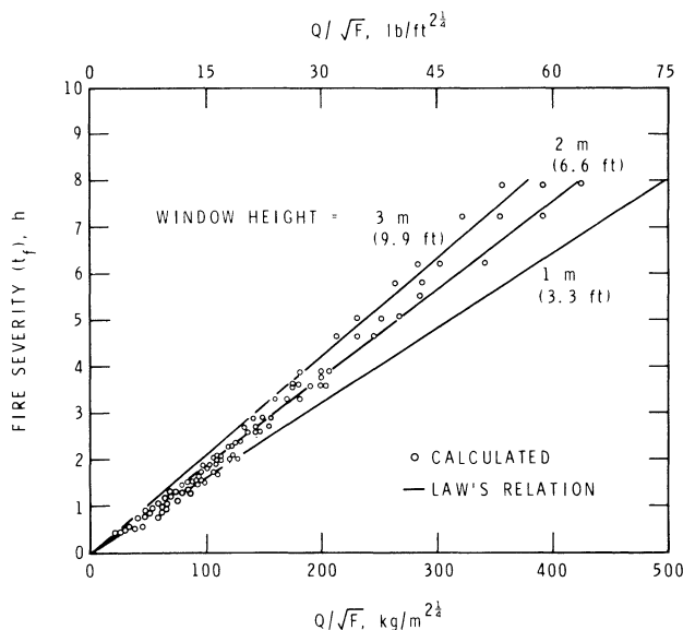
Fig. 11. Comparison of Law's relation with calculated values
