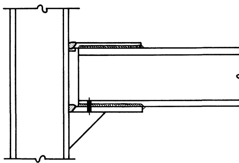
Fig. 24. Moment connection using flange connection plates. To avoid high shrinkage strains, beam seat is shop welded to column; top plate weld to column is made in field, followed by fillet welds of top and bottom plates to beam flanges.
