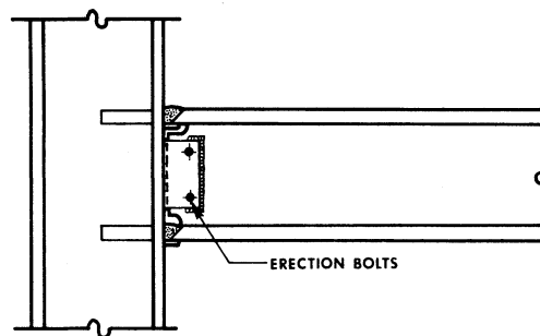
Fig. 23. Moment connection using shear connection plate. Welding plate to web after completion of flange welds avoids high shrinkage strains.
