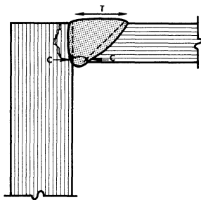
Fig. 14. Placing large welds close to the edge of a plate, as in the corner of a box column, increases susceptibility to lamellar tearing.
