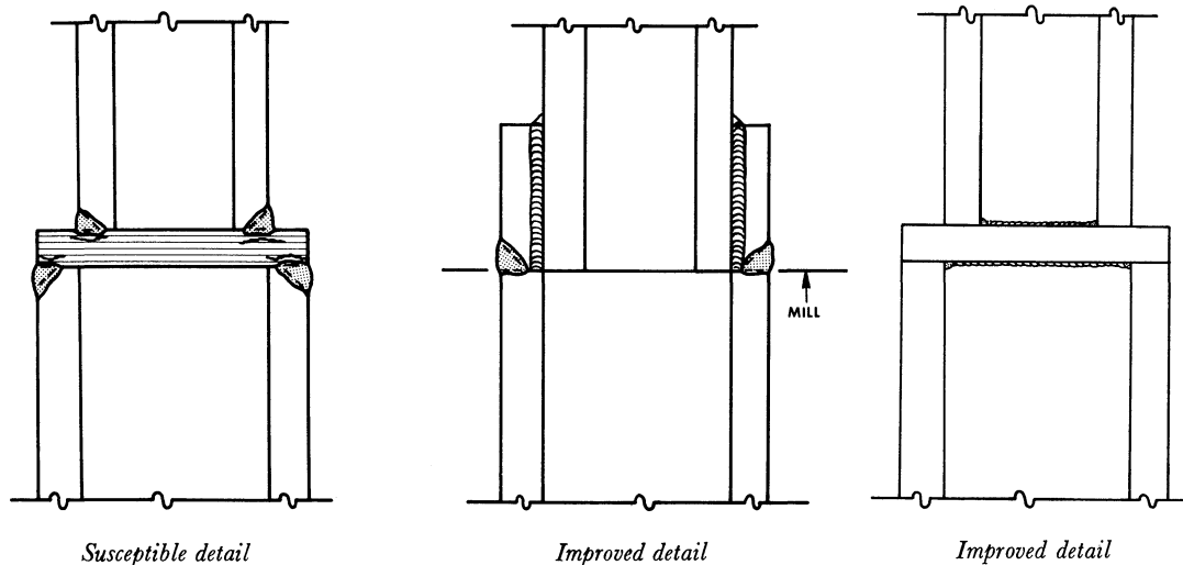
Fig. 25. Material susceptible to lamellar tearing can be eliminated by redesign of a connection.
