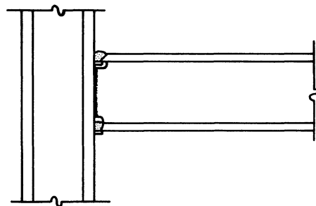
Fig. 12. Web welds and the thick column flanges provide high restraint to the contraction of large flange welds. Large unit strains are forced to concentrate in column flange opposite beam flange welds.
