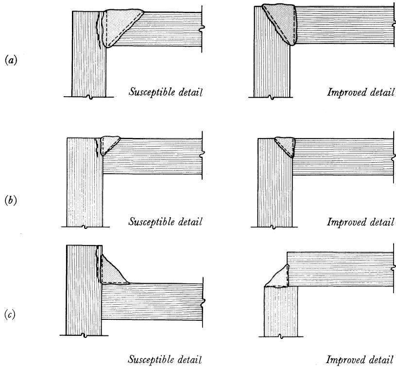
Fig. 26. Susceptibility to lamellar tearing can be reduced by careful detailing of welded connections.
