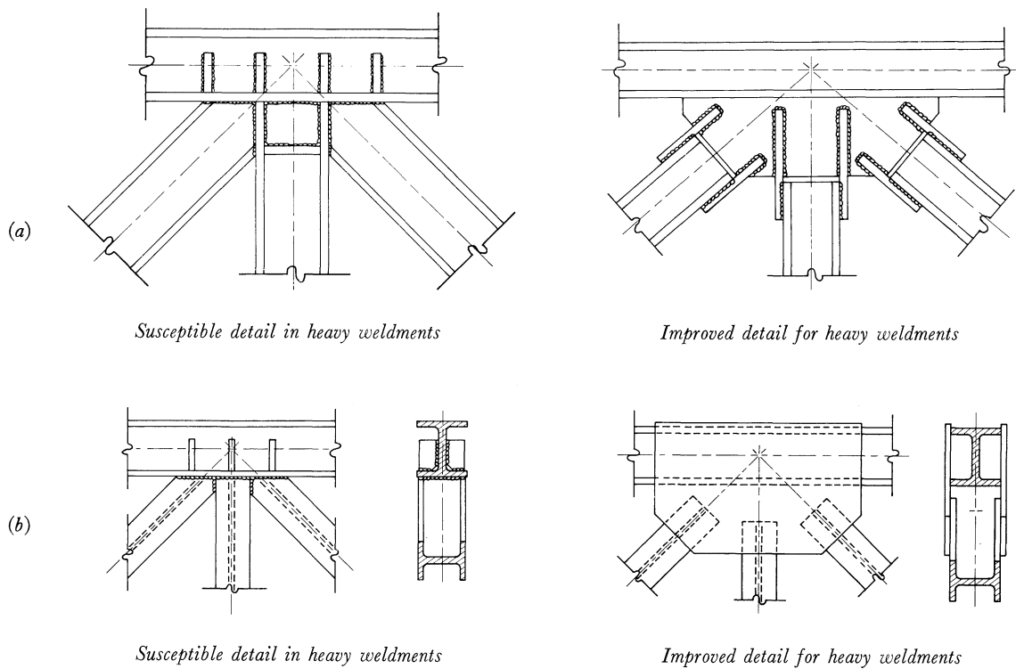
Fig. 27. In many cases large complex highly restrained connections can be redesigned to minimize or avoid joints which induce weld shrinkage strains in the thru-thickness direction of the connected material.
