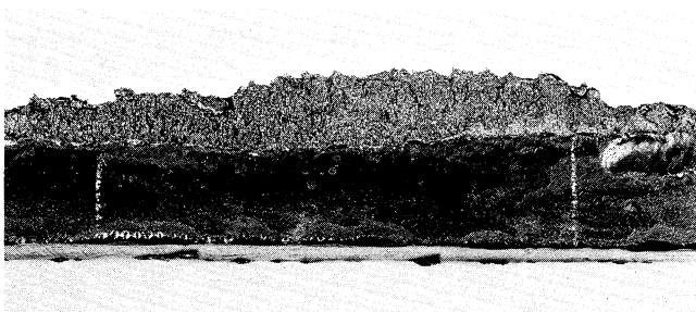
Fig. 6. Characteristic fibrous surface of lamellar tear
