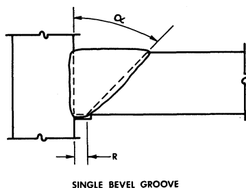
Fig. 20. Prequalified joints, such as AWS TC-U4a above, do not insure freedom from lamellar tearing.
