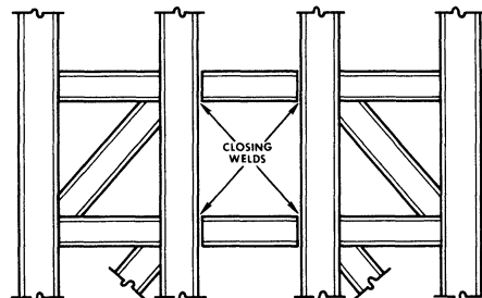
Fig. 19. Closing welds for members between rigid assemblies are subject to high restraint.
