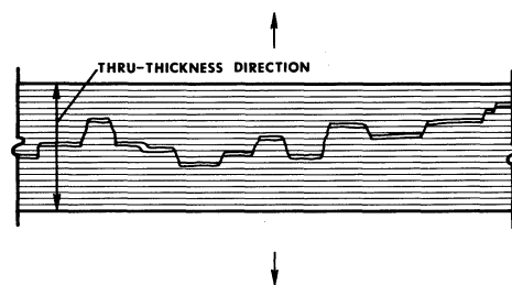
Fig. 8. Cross section of parent material showing complete development of the incomplete tear shown in Fig. 7
