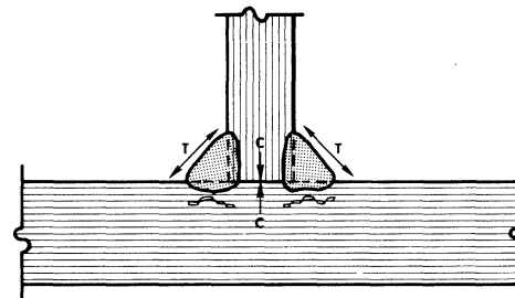
Fig. 17. Example of fit-up restraint with large double fillet welds
