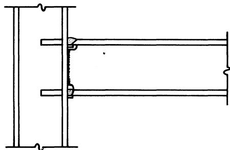
Fig. 13. Web welds and stiffened thin column flanges also provide high restraint to contraction of flange welds.
