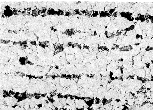
Fig. 11. Etched photomicrograph of banded microstructure in hot rolled steel (magnification 157X)
