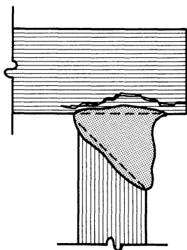
Fig. 15. Large volumes of weld metal increase susceptibility to lamellar tearing.
