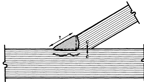
Fig. 16. Example of fit-up restraint with large single fillet weld
