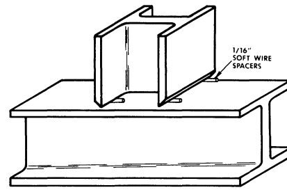
Fig. 28. Soft wire spacers permit welds to contract without inducing high strains in connected material.
