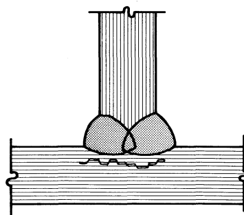
Fig. 1. Joint showing typical lamellar tear resulting from shrinkage of large welds in thick material under high restraint
