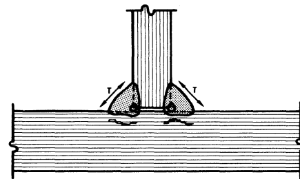
Fig. 18. Root passes of multiple pass welds restrain tee joints even when fit-up clearance is provided.
