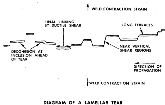
DIAGRAM OF A LAMELLAR TEAR
