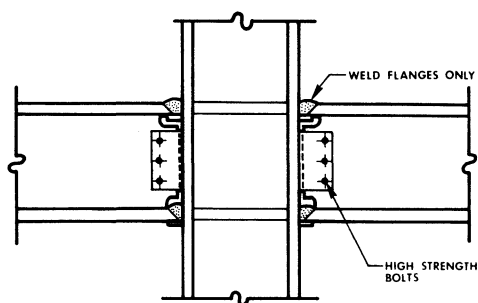
Fig. 22. Moment connection using shear connection plate. High strength bolted web connection allows flange weld shrinkage strains to be relieved.
