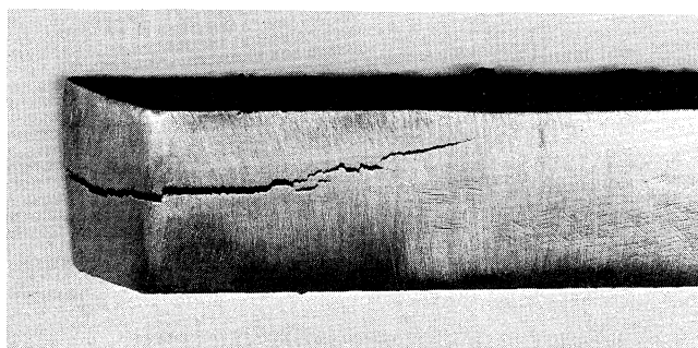
Fig. 5. Typical lamellar tear due to large thru-thickness strains. Note horizontal terraces with short vertical shear planes.
