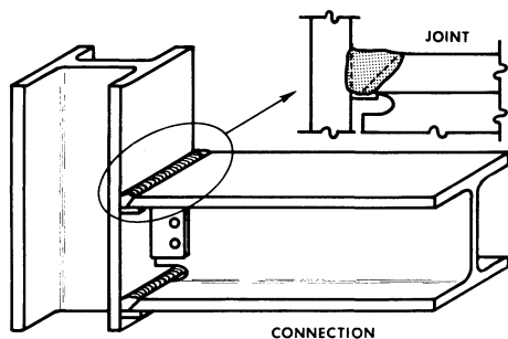
Fig. 2. Typical moment connection with full penetration welded flange joint
