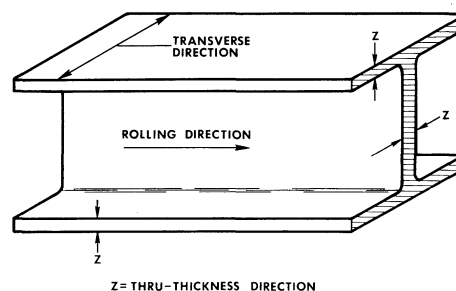
Fig. 3. Terminology related to rolling direction
