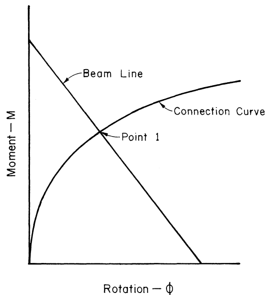
Fig. 3. Intersection of connection curve and "beam line" determines moment and rotation under gravity load condition
