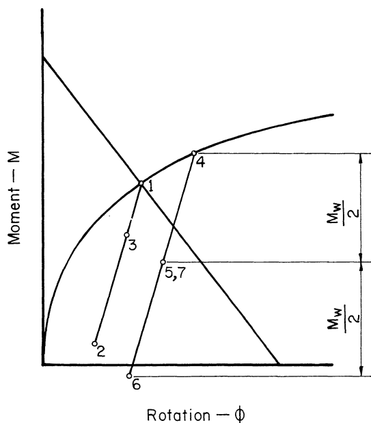
Fig. 6. History of Connection A when initial wind load is from left in the reverse directions from those indicated for Connection A.
