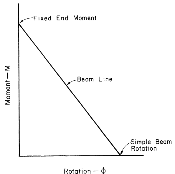
Fig. 2. "Beam line" for a uniformly loaded girder
