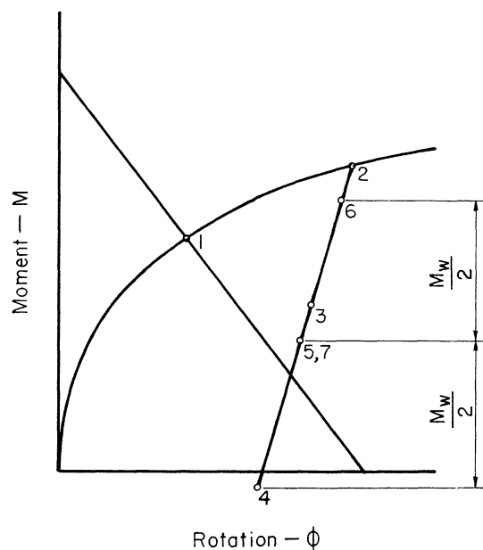
Fig. 5. History of Connection A when initial wind load is from right
