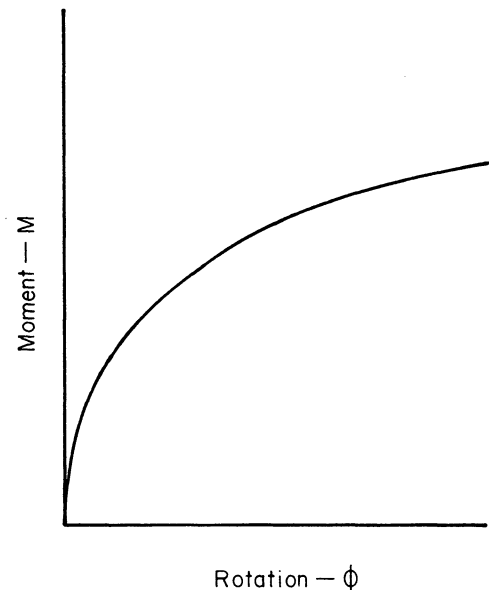
Fig. 1. M - \phi curve for a typical moment connection
