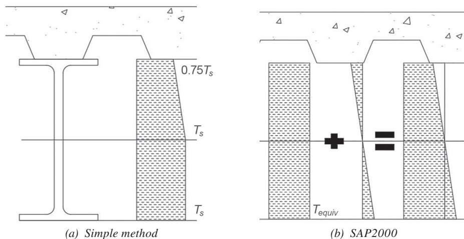
Fig. 9. Thermal gradient across composite beam section.
