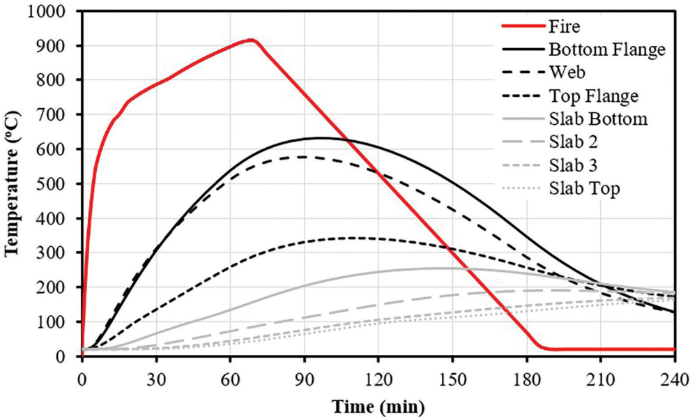
Fig. 7. Time-temperature response of W14×22 composite beam with 1-hr FRR fire protection exposed to fire.
