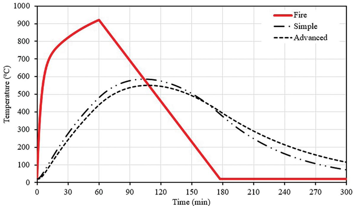
Fig. 8. Results of lumped heat capacity analysis for W12×58 column.
