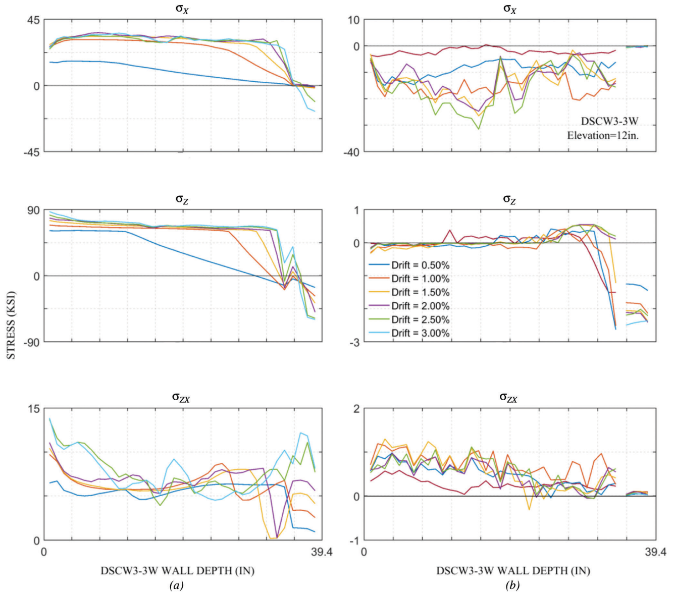
Fig. 23. Plane stress distribution of the cross section of the LS-Dyna model of DSCW3-3W located at 12-in. wall height under negative drift: (a) shell stress distribution in steel skin; (b) average solid stress distribution in concrete.
