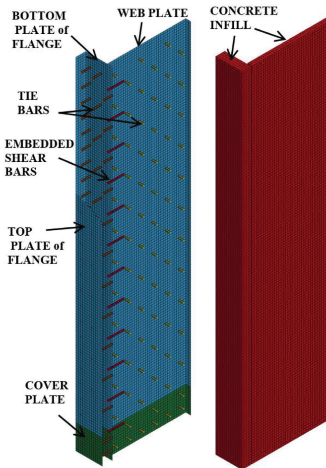
Fig. 12. LS-Dyna model of the half-symmetric T-Wall DSCW3.
