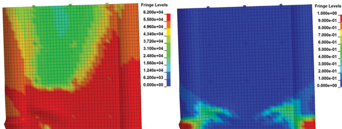
Fig. 6. Von Mises yield stress (a) and effective plastic strain (b) contours of the LS-Dyna model for CFSSP-B2 at 3.33% drift.
