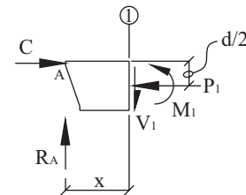
Fig. 9. Free-body diagram along zone 1.
