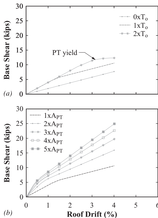
Fig. 15. PT boundary frame: (a) T_0 variable; (b) A_{PT} variable.
