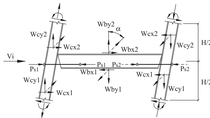
Fig. 3. Resultant force free-body diagram.
