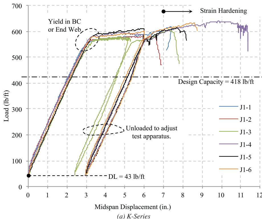
Fig. 3. Load-displacement results: (a) K-series (continued next page).
